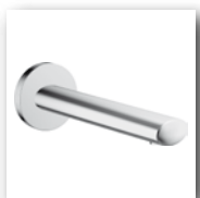
HANSARONDA Bathtub spout, DN 15 (G 1/2) 0582 2172 chrome Projection: 180 mm
