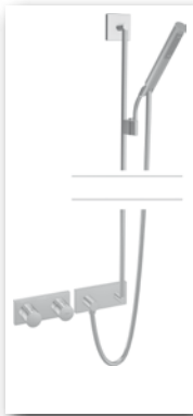
HANSAMATRIX Trim kit installation pack 05 thermostat mixer, DN 15 (G1/2)* 4487 0050 chrome suitable for HANSADESIGNO, HANSALIGNA, HANSASTELA, HANSARONDA with wall bar kit
