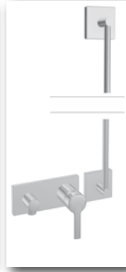
HANSAMATRIX Trim kit installation pack 01 single-lever mixer, DN 15 (G1/2)* 4487 2010 chrome suitable for HANSARONDA with all-metal wall bar 1100 mm
